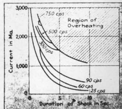
FIG. 7—Minimum currents necessary to cause death from shocks of different duration at several frequencies
