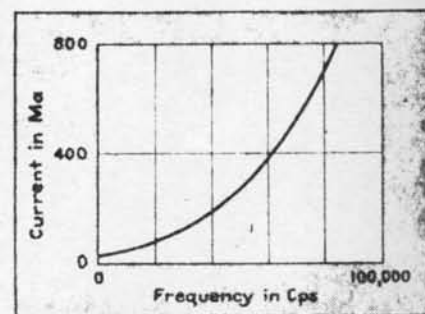
FIG. 6—Effect of frequency on tolerance current
